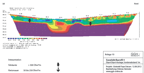
Geoelectrical section 4, the 'dromos' in the bedrock is clearly visible (graphics: GGH).
